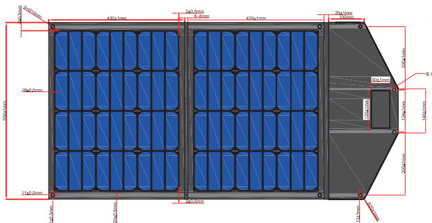
Fully expanded
